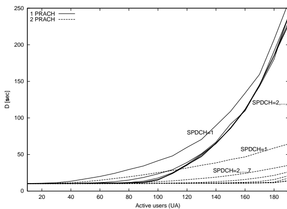
Figure 5: Plots of D in scenario 1
