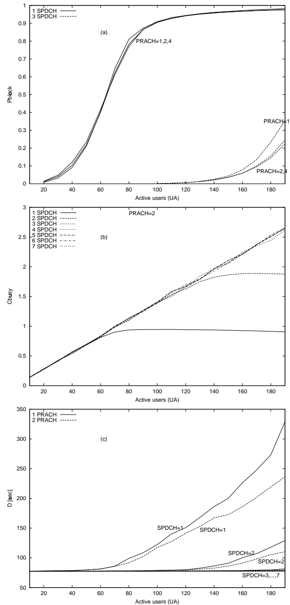
Figure 6: Plots of P_{block} (a), C_{busy} (b) and D (c) in scenario 2
