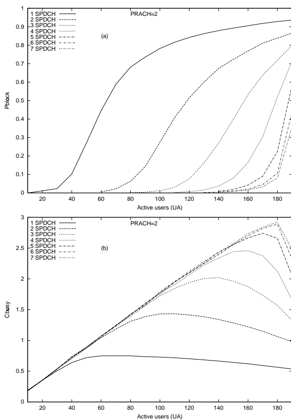
Figure 3: Plots of P_{block} (a) and C_{busy} (b) in scenario 1
