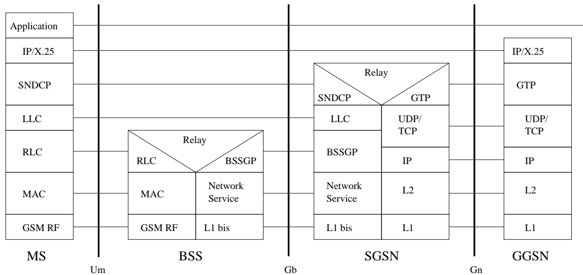
Figure 1: The ISO/OSI structure of GPRS
