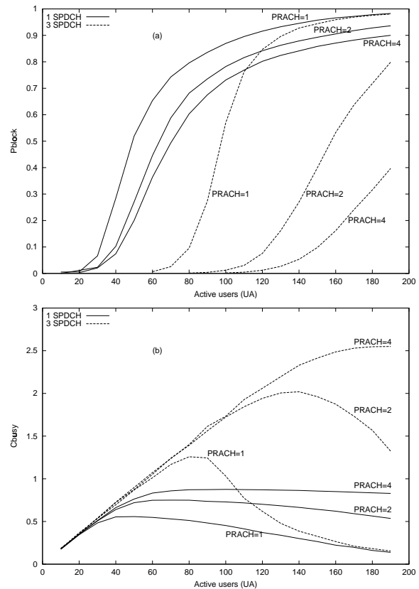
Figure 4: Plots of P_{block} (a) and C_{busy} (b) in scenario 1
