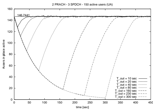
Figure 7: Recovery from outages
